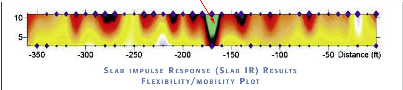
Evidence of water infiltration causing bulging Mechanically Stabilized Earth (MSE) wall correlates to area of high relative mobility.
