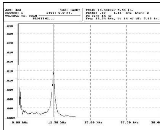
Fig. 3d Accelerometer Spectral Response on a Slab, Integrated to Displacement
